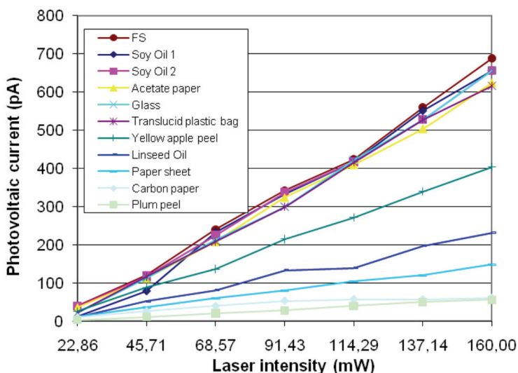
Fig. 13. CCP detected curves from different liquids and thin solids
