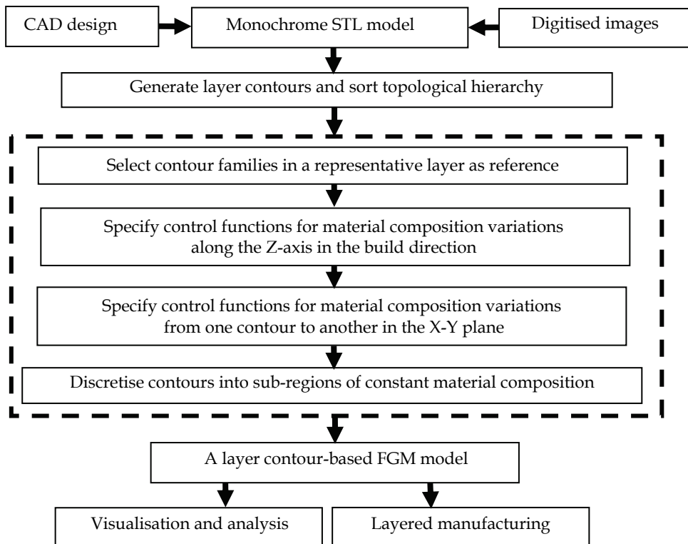
Fig. 8. The flow of processing FGM objects
