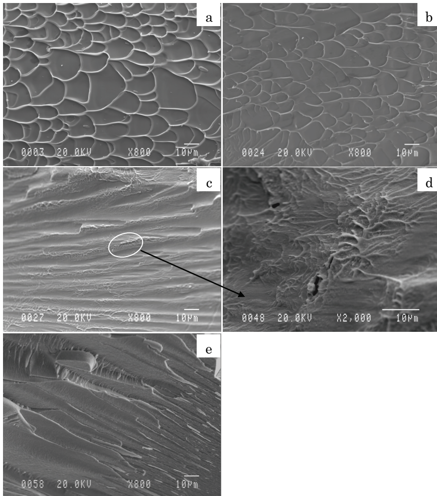
Fig. 6. Fracture morphologies of the Ti_{40}Zr_{10}Cu_{36}Pd_{14} bulk metallic glass and its annealed alloys: as-cast (a), annealed at 693K (b), 723 K (c) (d), and 823 K (e) for 10 min.
