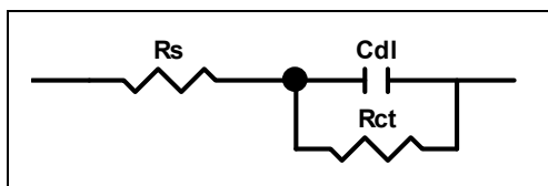
Fig. 3. Equivalent Electric Circuit (Randless) of the electrode-electrolyte interface.
