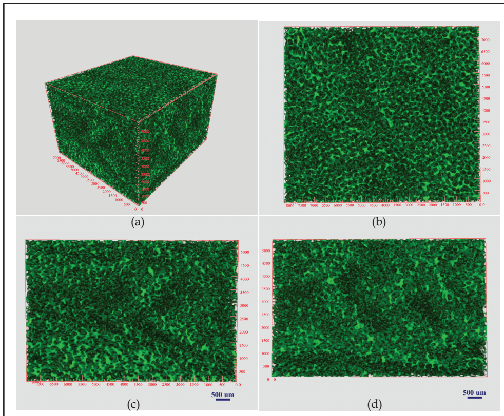
Fig. 8. Micro-CT 3D reconstructions of the Ti foam with NaCl as spacer material prepared by SPS at 700 °C under 50 MPa with an isometric view (a), 2D top view (b), left side view (c), and right side view (d). Scale spacing, 500 \mu\text{m} .
