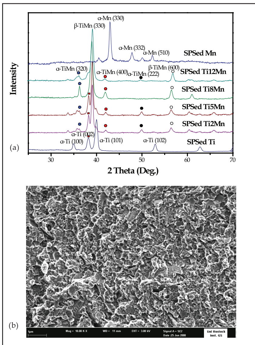
Fig. 4. XRD patterns of the spark plasma sintered Ti, Mn and TiMn alloys showing the TiMn alloys are \alpha+\beta phase alloy (a) and SEM micrograph of the fracture surface of a Ti8Mn alloy.
