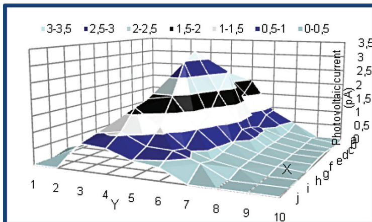
Fig. 12. CCP curve response without sample when is stimulated 160 \text{ mW}/\text{cm}^2 of LASER illumination
