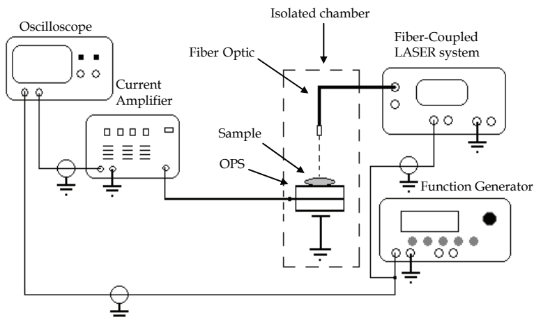
Fig. 11. Experimental setup for opacity measure
