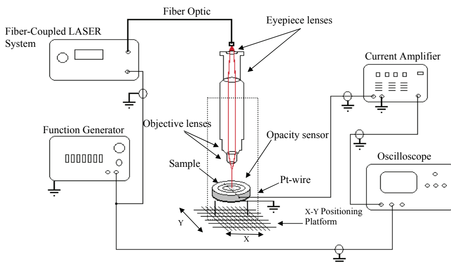
Fig. 14. Experimental setup used as 2D opacity scan
