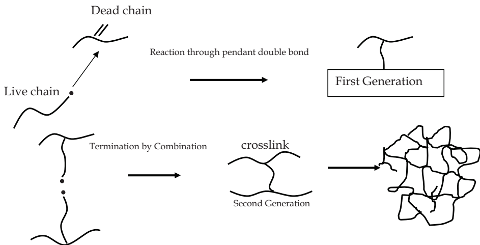
Scheme 3. Reactions leading to gel formation.
