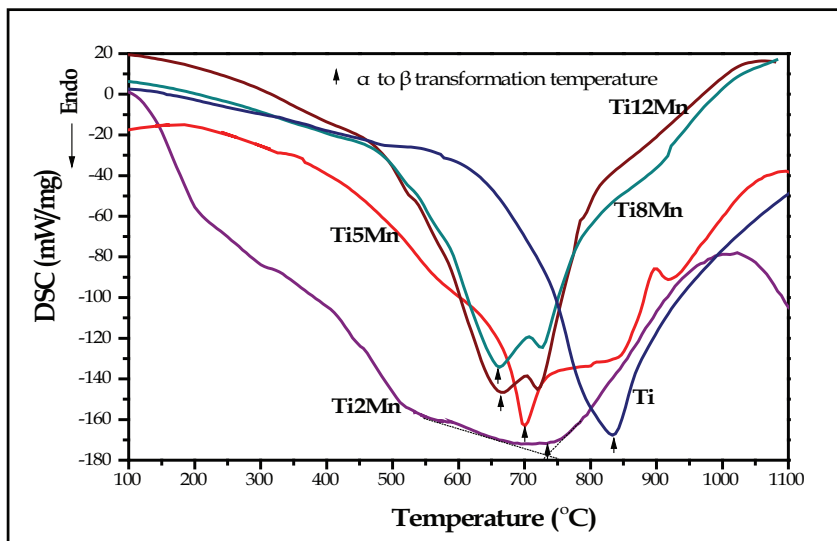
Fig. 3. Phase transformation behaviours of the TiMn alloys measured by DSC showing the decrease of the \alpha to \beta transformation temperatures with increasing Mn amount.
