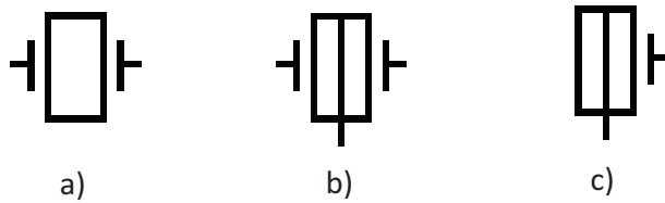
Fig. 2. Graphical symbols that represent reference piezoceramic of PLZT and CCP a) reference piezoceramic with two electrodes, b) CCP, with implant of Pt-wire and two electrodes, c) CCP without an electrode which side face is used like sensor
