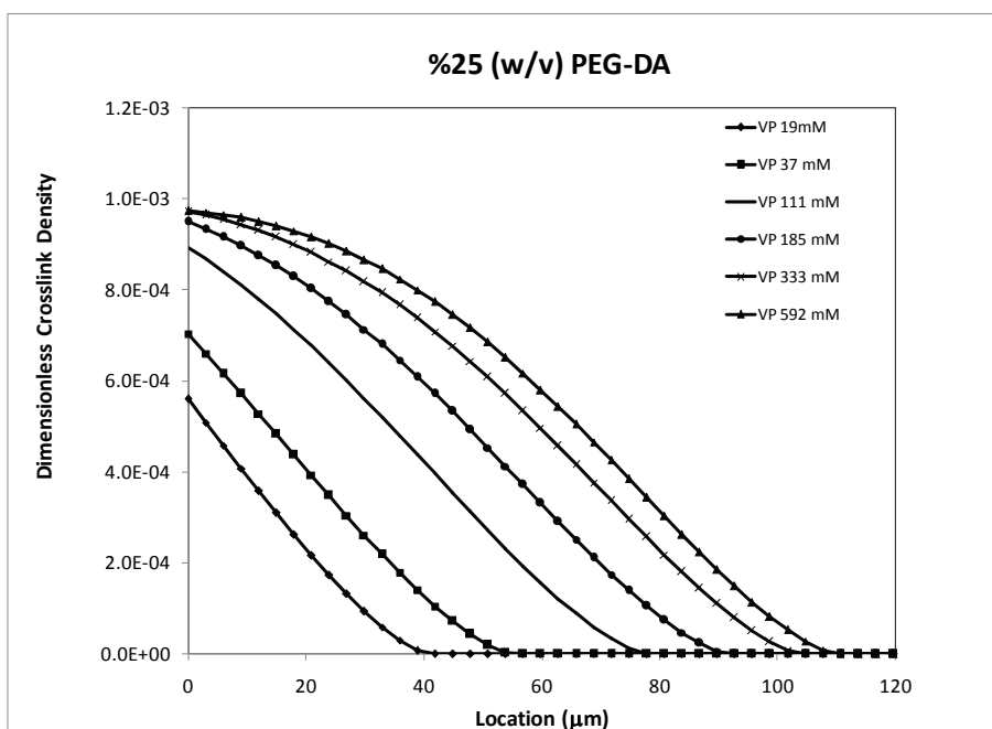
Fig. 5. Effect of concentration changes of VP on the dimensionless crosslink density versus location of GLP-1 functionalized PEG hydrogel membrane ( [\text{TEA}] = 225 \text{ mM} , [\text{acrl-PEG-GLP-1}] = 14.8 \mu\text{M} ), 25% (w/v) PEG-DA in prepolymer solution.
