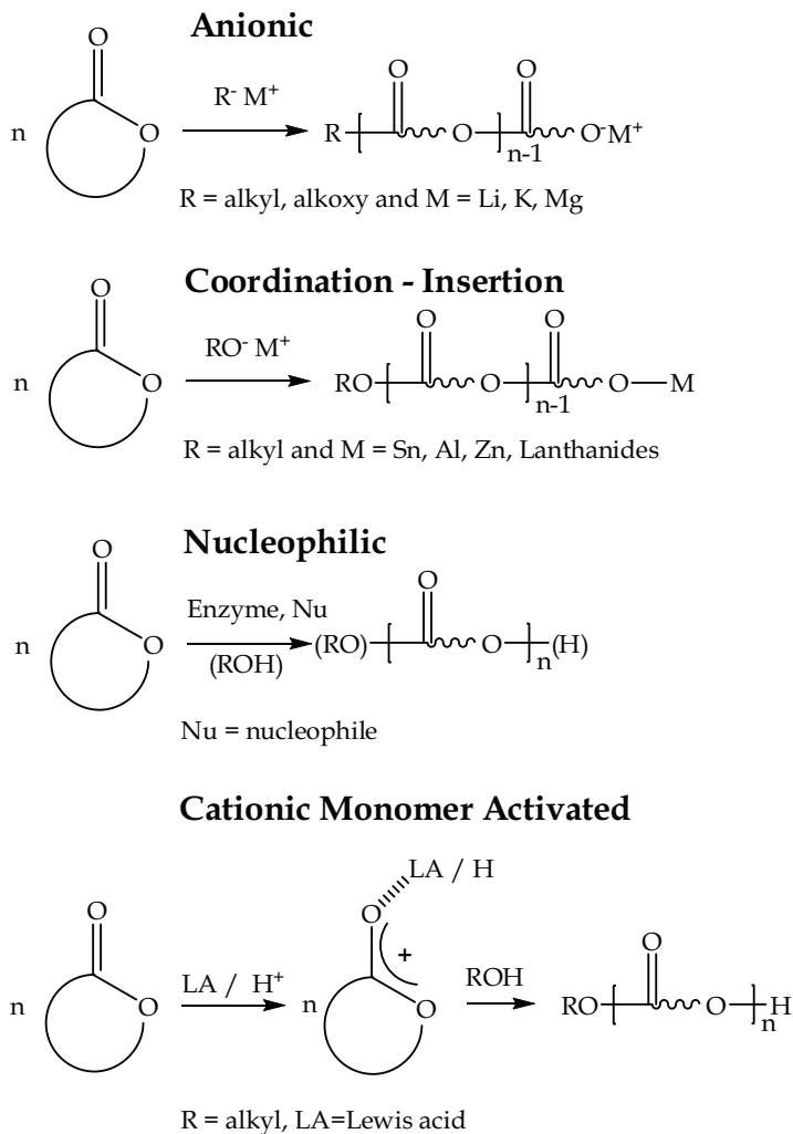
Fig. 2. Ring-opening polymerization mechanisms
