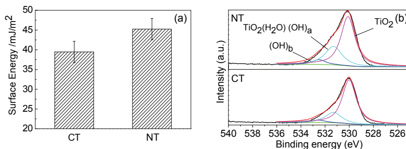
Fig. 24. (a) Comparison of surface energy of CT and NT samples; (b) x-ray photoelectronic spectrum O 1s peaks obtained from CT and NT samples (Zheng, 2009).
