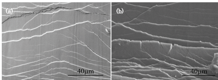
Fig. 8. Lateral surface of the (\text{Ti}_{40}\text{Zr}_{10}\text{Cu}_{36}\text{Pd}_{14})_{100-x}\text{Nb}_x as-cast rods after fracture (a) x=1 , (b) x=3 .
