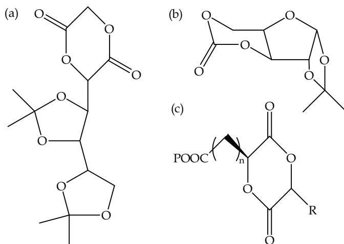
Fig. 16. Examples of carbohydrate derived monomers : 3-(1,2,3,4-tetraoxobutylidene)isopropylidene)dioxane-2,5-dione ((a), Benabdillah et al., 1999), 1,2-isopropylidene-[D]-xylofuranose-3,5-cyclic carbonate ((b), Chen & Gross, 1999) and 1,4-dioxane-2,5-diones featuring pendant carboxyl groups (P = protecting group, x=1 , R=CH_2COOP ; x=1 , R=H ; x=2 , R=CH_3 , Thillaye du Boulay et al., 2008)
