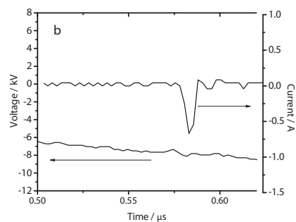
Fig. 7. Current-voltage characteristics for glass composite electrode at 1 mm inter-electrode distance with different time resolution
