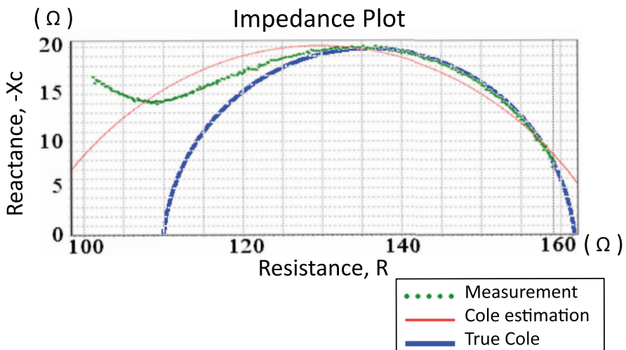
Fig. 3. Typical impedance plot of a measurement showing data deviation caused by a capacitive leakage.
