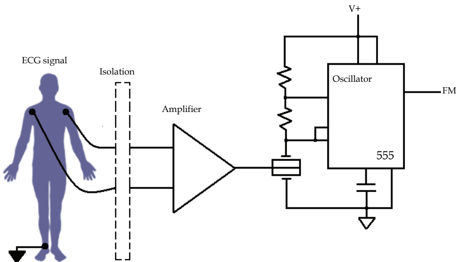
Fig. 5. CCP used as frequency modulator
