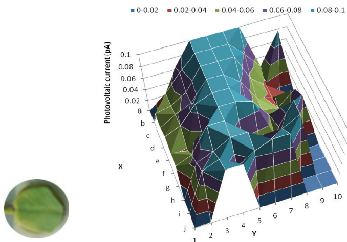
Fig. 15. CCP response with a plant leaf
