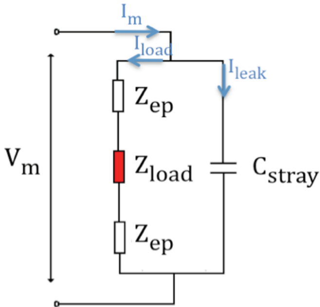
Fig. 2. Electrical equivalent of a EBI measurement setup with a parasitic capacitance in parallel with the impedance load.
