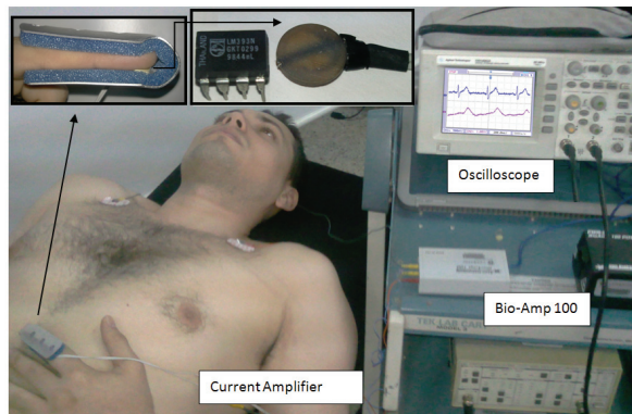
Fig. 8. Real setup used for get fingertip pulses
