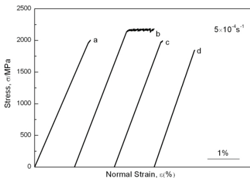
Fig. 5. Compressive strain-stress curves of the Ti 40 Zr 10 Cu 36 Pd 14 bulk metallic glass and its annealed alloys: as-cast (a), annealed at 693 K (b), 723 K (c) and 823 K (d) for 10 min
