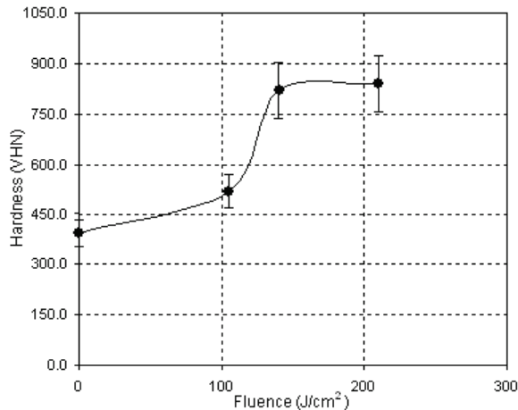
Fig. 12. Variation of surface hardness with fluence
