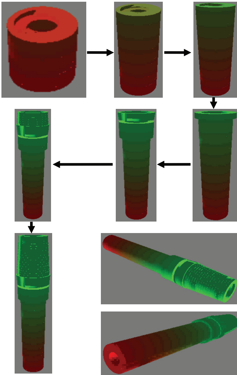
Fig. 20. Digital fabrication of a multi-material prototype of a dental implant assembly
