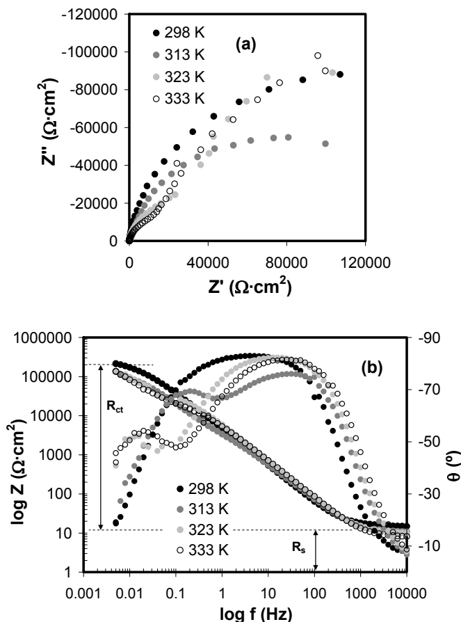
Fig. 7. (a) Nyquist diagrams and (b) Bode plots of a CoCrMo alloy at OCP in NaCl+50 mg/L BSA at different temperatures and pH 7.4 (Valero & Iguar, 2010).
