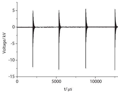
Fig. 6a. Profile of high voltage pulses
