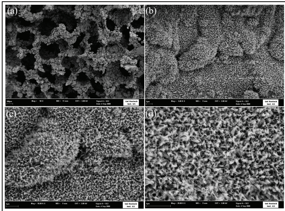
Fig. 12. SEM micrograph of the Ti8Mn foams prepared by the SPS and NaCl dissolution method (a), and morphologies of the surface modified \text{TiO}_2 nanostructures on the porous wall of the foams at different magnifications (b-d).
