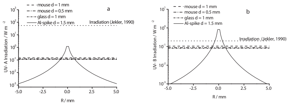
Fig. 11. Simulated UV-A (a) and UV-B (b) irradiation of treated surface for different electrode and irradiation according to (Jekler, 1990).
