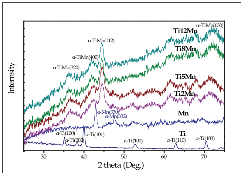
Fig. 2. XRD patterns of the Ti, Mn powders, and TiMn alloy powders prepared by mechanical alloying showing the formation of \alpha -TiMn phases.
