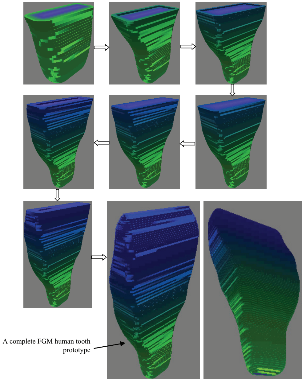
Fig. 23. Digital fabrication of an FGM human tooth
