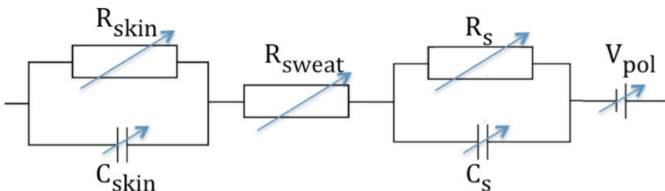
Fig. 1. Electrical Equivalent of the Skin-Electrode Interface
