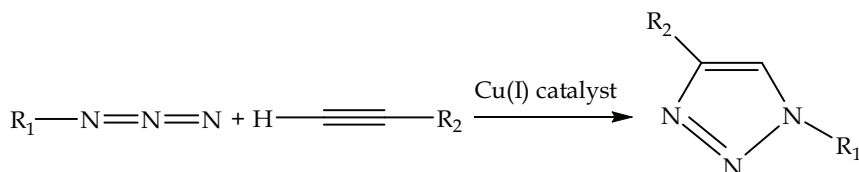
Fig. 17. Copper(I)-catalyzed alkyne-azide cycloaddition
