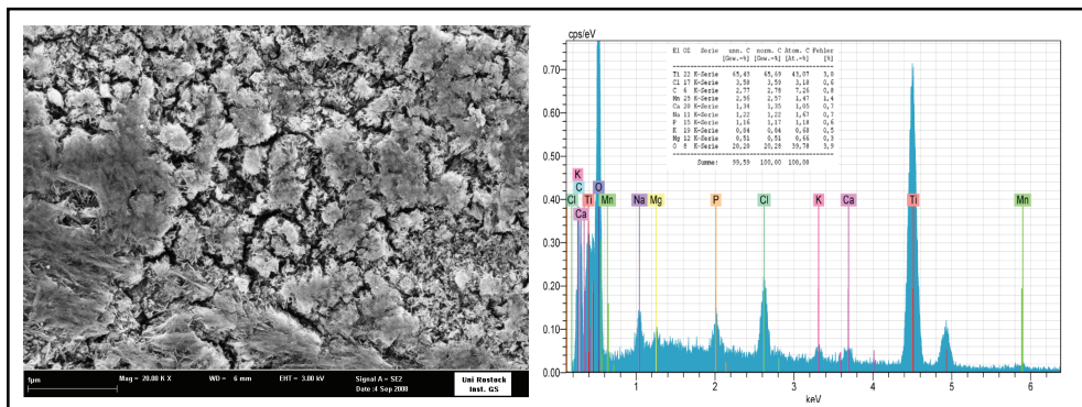
Fig. 13. SEM micrograph (a) and EDX (b) of the \text{TiO}_2 modified Ti8Mn foam immersed in simulated body fluid for 3 days showing the apatite formation.
