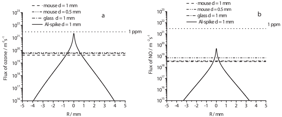
Fig. 10. Flux of ozone (a) and nitric oxide (b) reaching the treated surface across the radius of the driving electrode ( R ) for DBD on different substrates. The fluxes at species' concentration of 1 ppm are calculated using mean velocity and concentration of nitrogen and oxygen molecules at plasma conditions.
