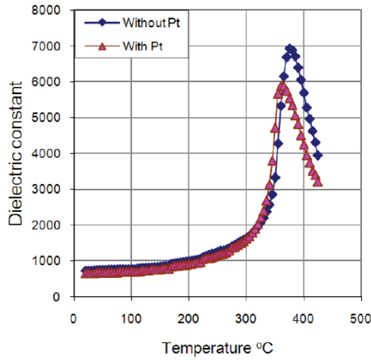
Fig. 1. Dielectric constant piezoelectric ceramic PLZT
