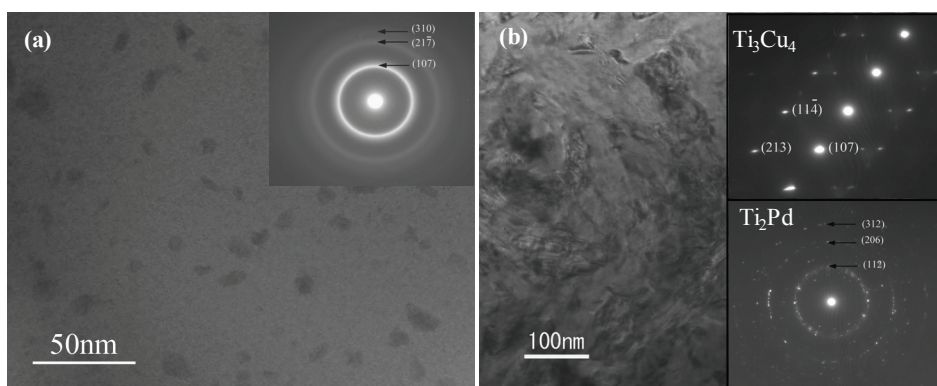
Fig. 4. Bright field TEM images and corresponding selected area diffractions of the Ti_{40}Zr_{10}Cu_{36}Pd_{14} alloys annealed at 723 K (a) and 823 K (b).
