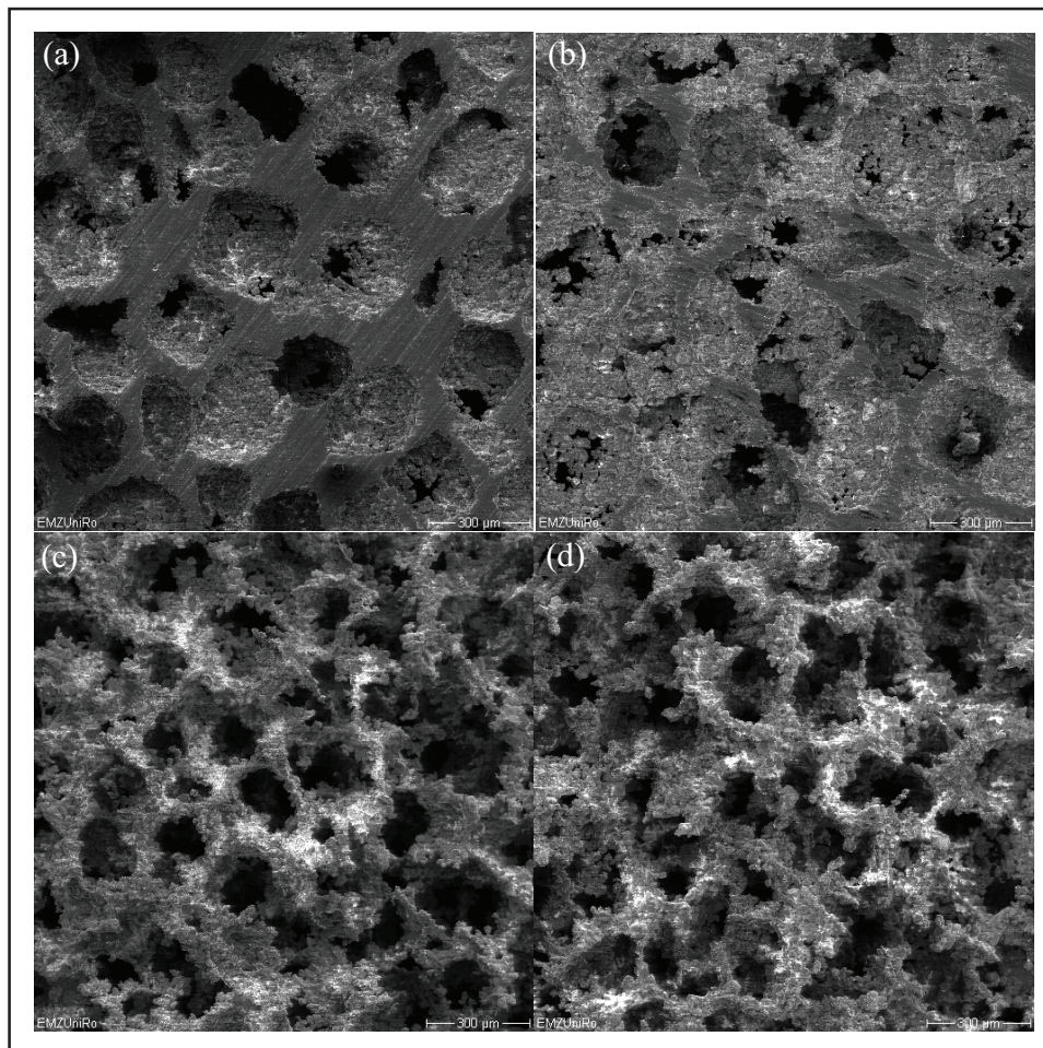
Fig. 10. SEM micrographs of the Ti foams with the same pore size of 250 μm but different porosities of 30 % (a), 45% (b), 55% (c) and 70% (d). Scale bars, 300 μm.
