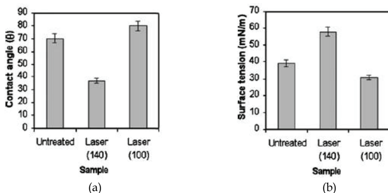
Fig. 16. Variation of contact angle: (a) and surface tension, (b) with sample surface texture
